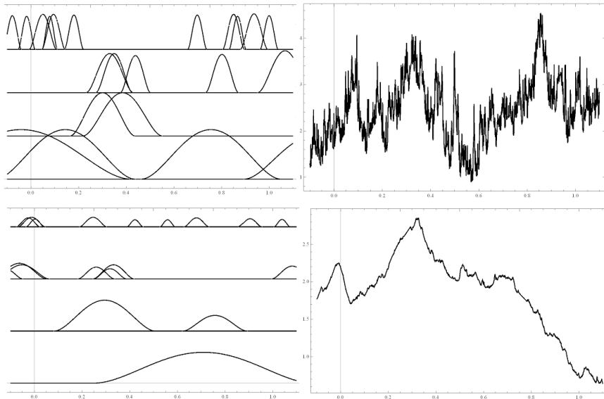
FIGURE 1. Two sample paths obtained with different pulses and parameters
