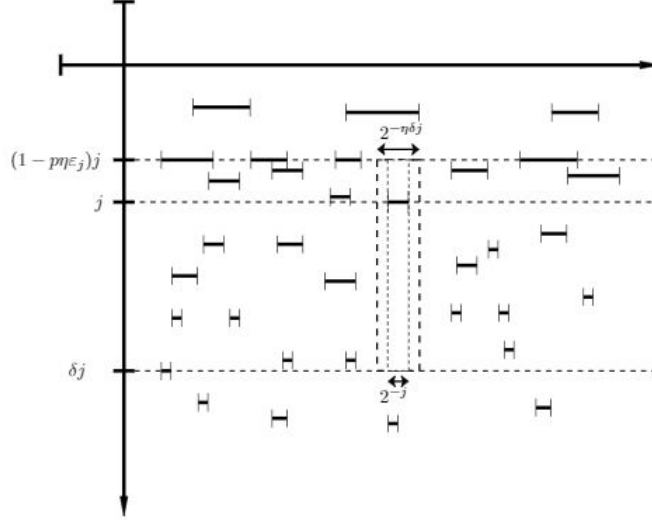
FIGURE 4. Representation of pulses supports in \mathcal{I}_j .
