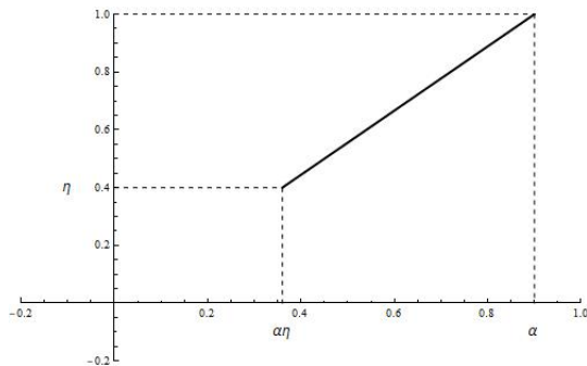
FIGURE 3. Multifractal spectrum in the case \alpha = 0.9 and \eta = 0.4
