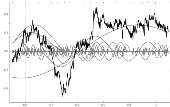
FIGURE 2. Sample path of F computed with 1000 dilated and translated pulses
